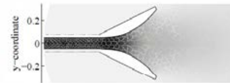
FIGURE 12: The square of the absolute value of the sound pressure distribution at 550 Hz after optimization. Note that the banded structure in the waveguide shown in figure 8 has disappeared.
