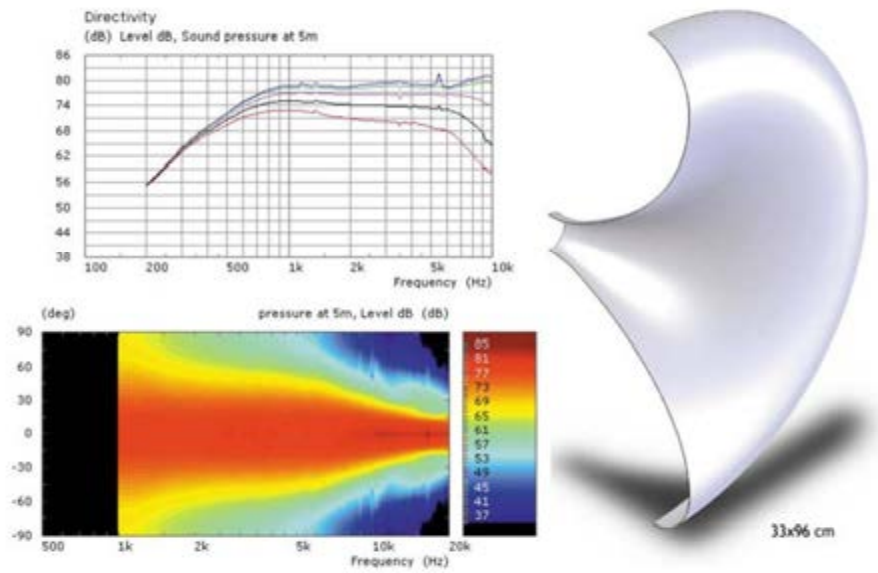
Minimum phase horns (or short Minphase) by ing. Michael Gerstgrasser. This are state-of-the-art Gauss optimized horns that offer smoothest sound field with controlled directivity (CD) and good look. Above example with a flat 3" diaphragm.
