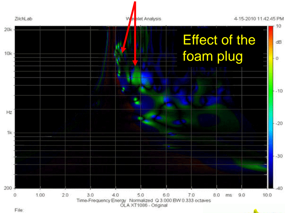
subtraction of the wavelets graph of the OSWGD without its foam plug and with its foam plug
