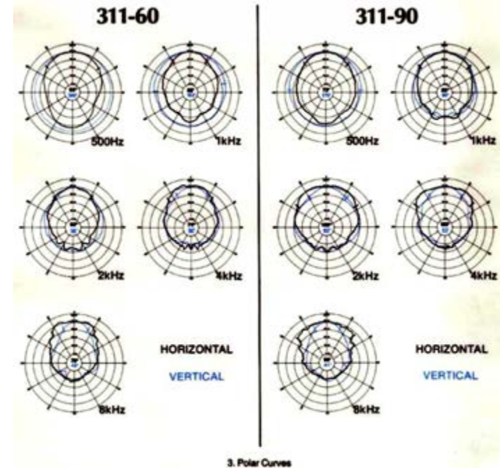
3. Polar Curves
