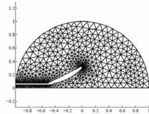
FIGURE 7: The finite element mesh, denoted Mesh I in table 2, on the initial geometry. Note that the \Gamma_d^{int} is different from \Gamma_d^{ref} .
