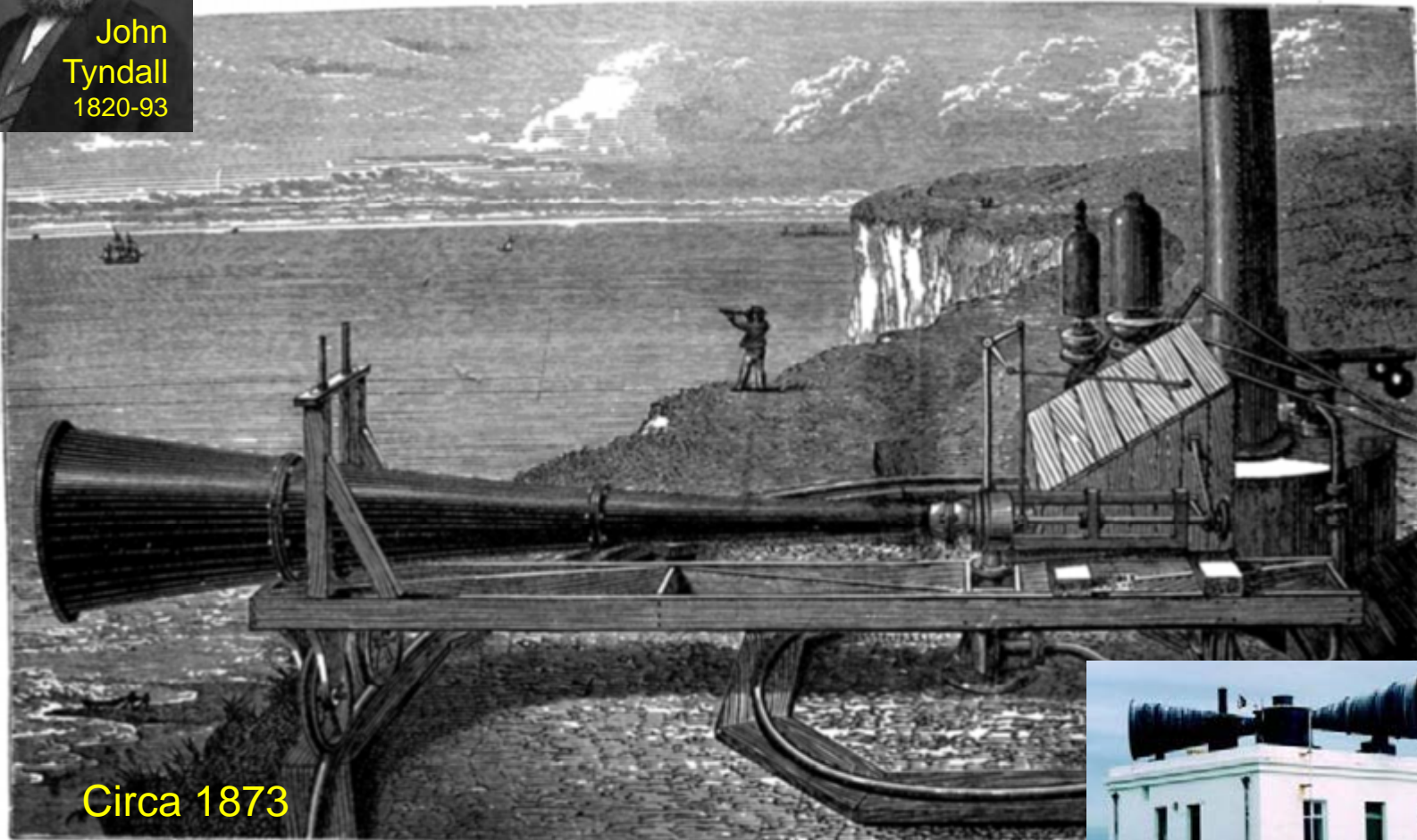
Tyndall's fog-horn
